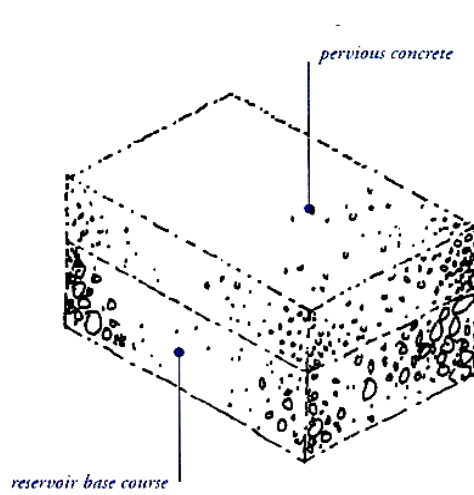
Pervious concrete
