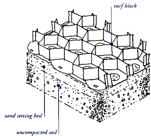
Turf block
