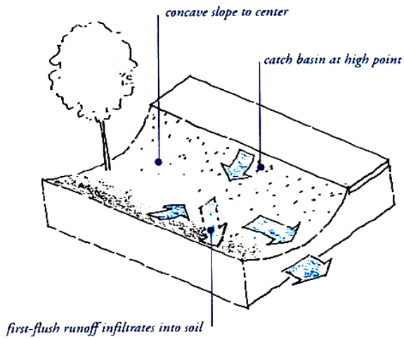
Concave median
